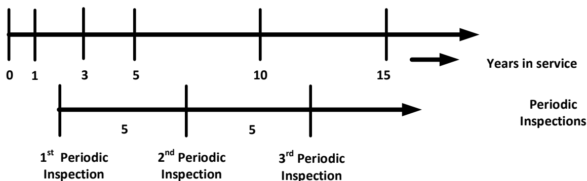
Figure 1 Example of acetylene cylinder test programme
